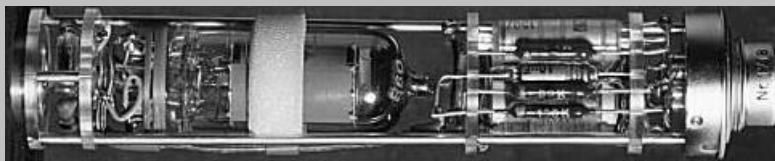
Open amplifier without capsule: The 6AU6 valve
