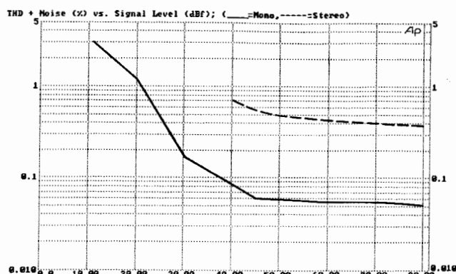
Fig. 2—THD + N vs. signal strength at 1 kHz for wide (A) and narrow (B) i.f. modes.
