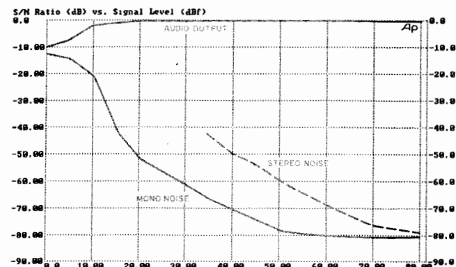
Fig. 1—Mono and stereo quieting characteristics, wide i.f. mode, for "Single r.f." (A) and "Double r.f." (B) settings.
