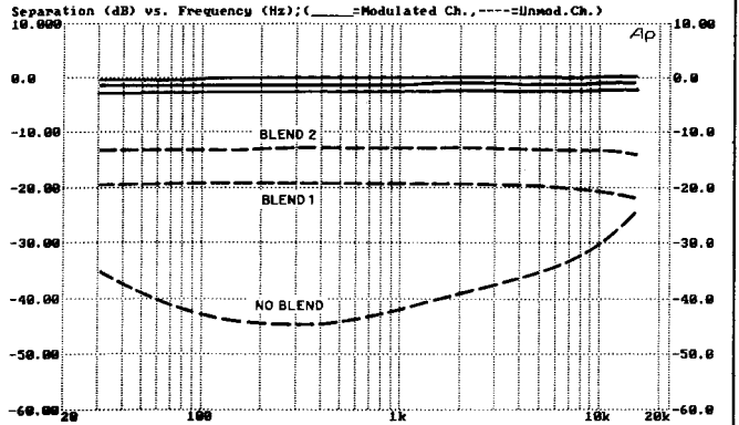
Fig. 4—FM frequency response (solid curves) and separation vs. frequency (dashed curves) for wide (A) and narrow (B) i.f. modes. Note the two blend levels. Solid curves are output with (top to bottom) no blend, Blend 1, and Blend 2.
