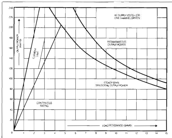
Fig. 1 Power output versus time and load impedance
